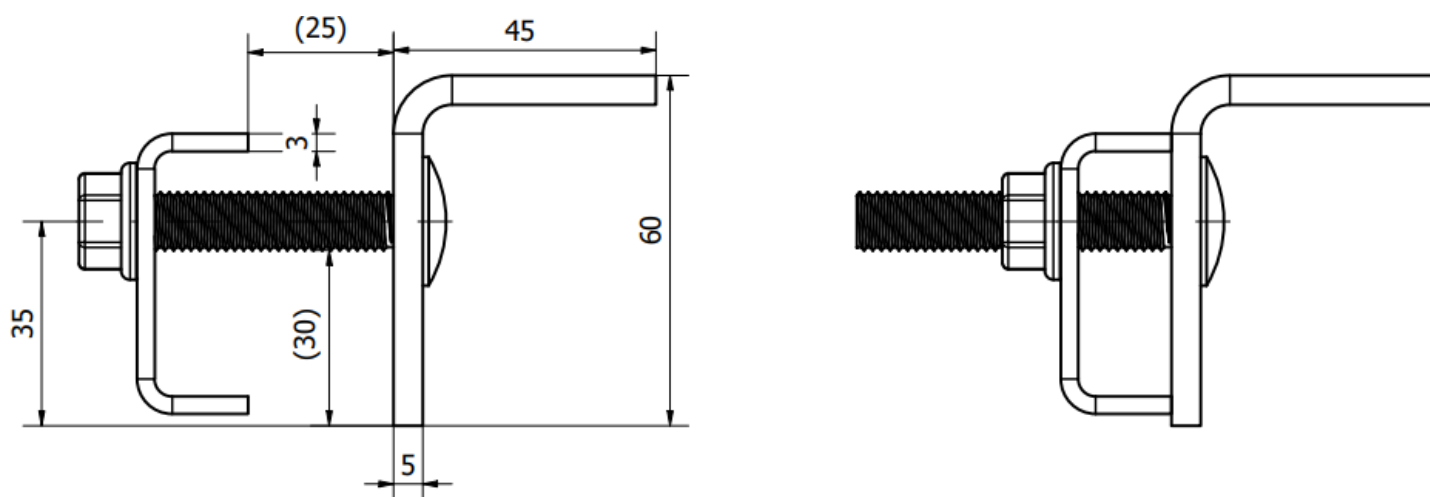
Fig.1 dimensions of K-24-U
